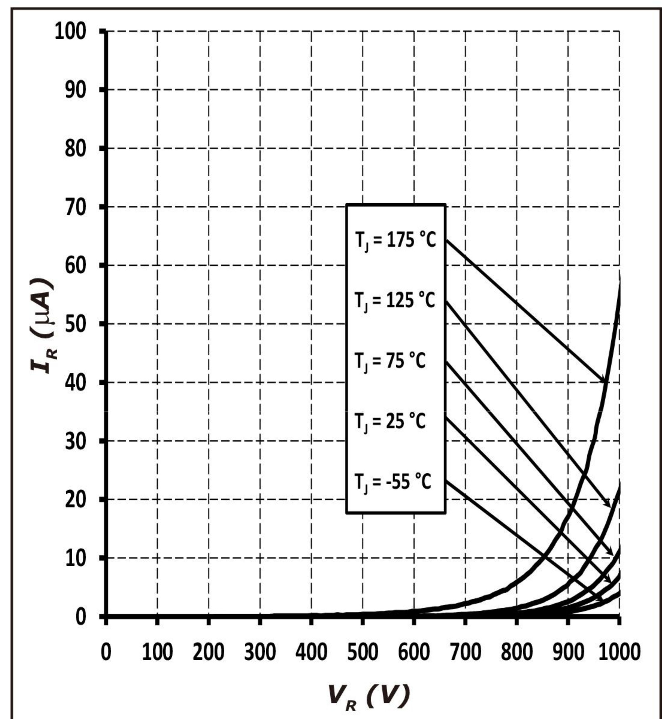
Figure 2. Reverse Characteristics
