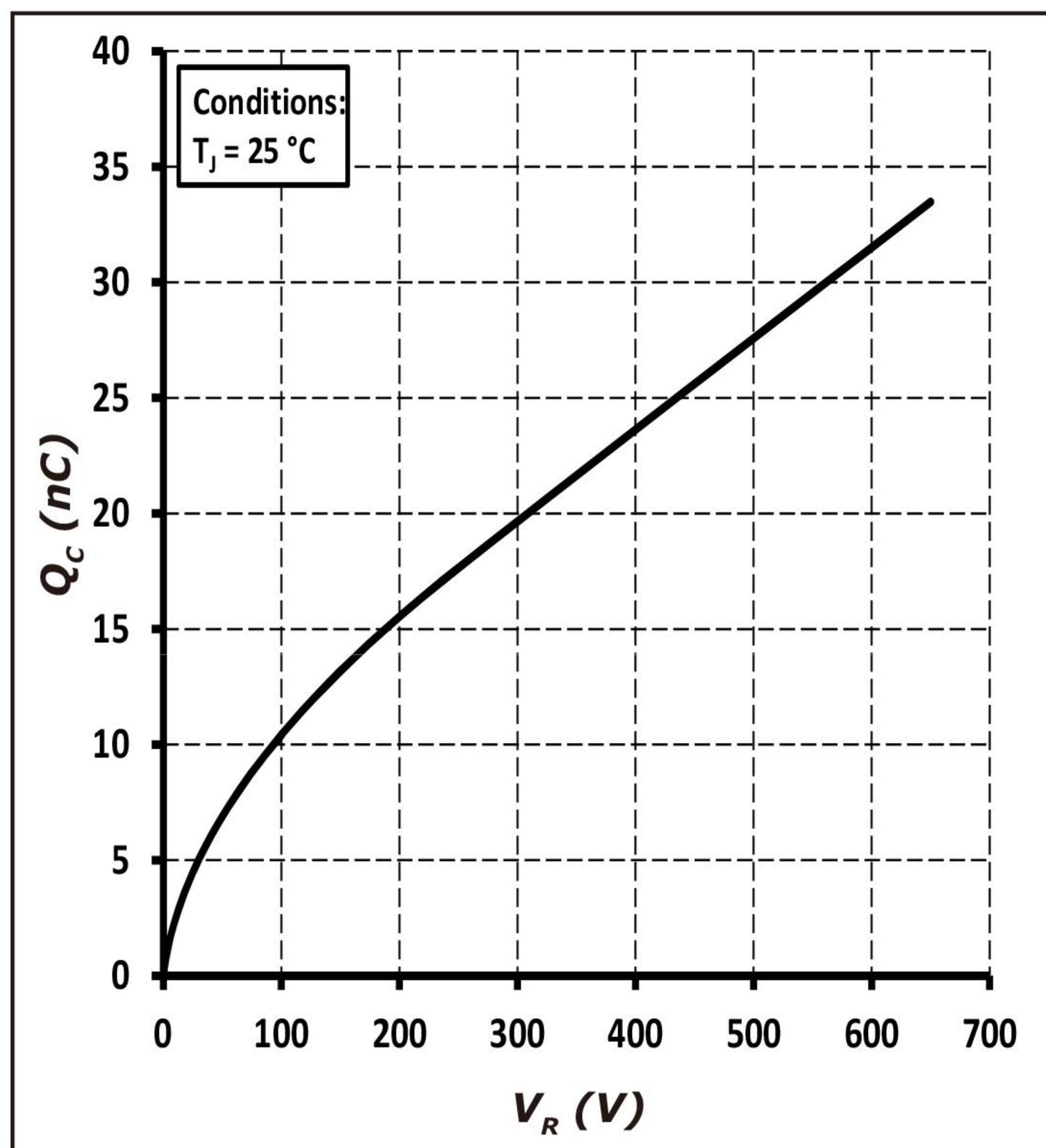
Figure 5. Total Capacitance Charge vs. Reverse Voltage
