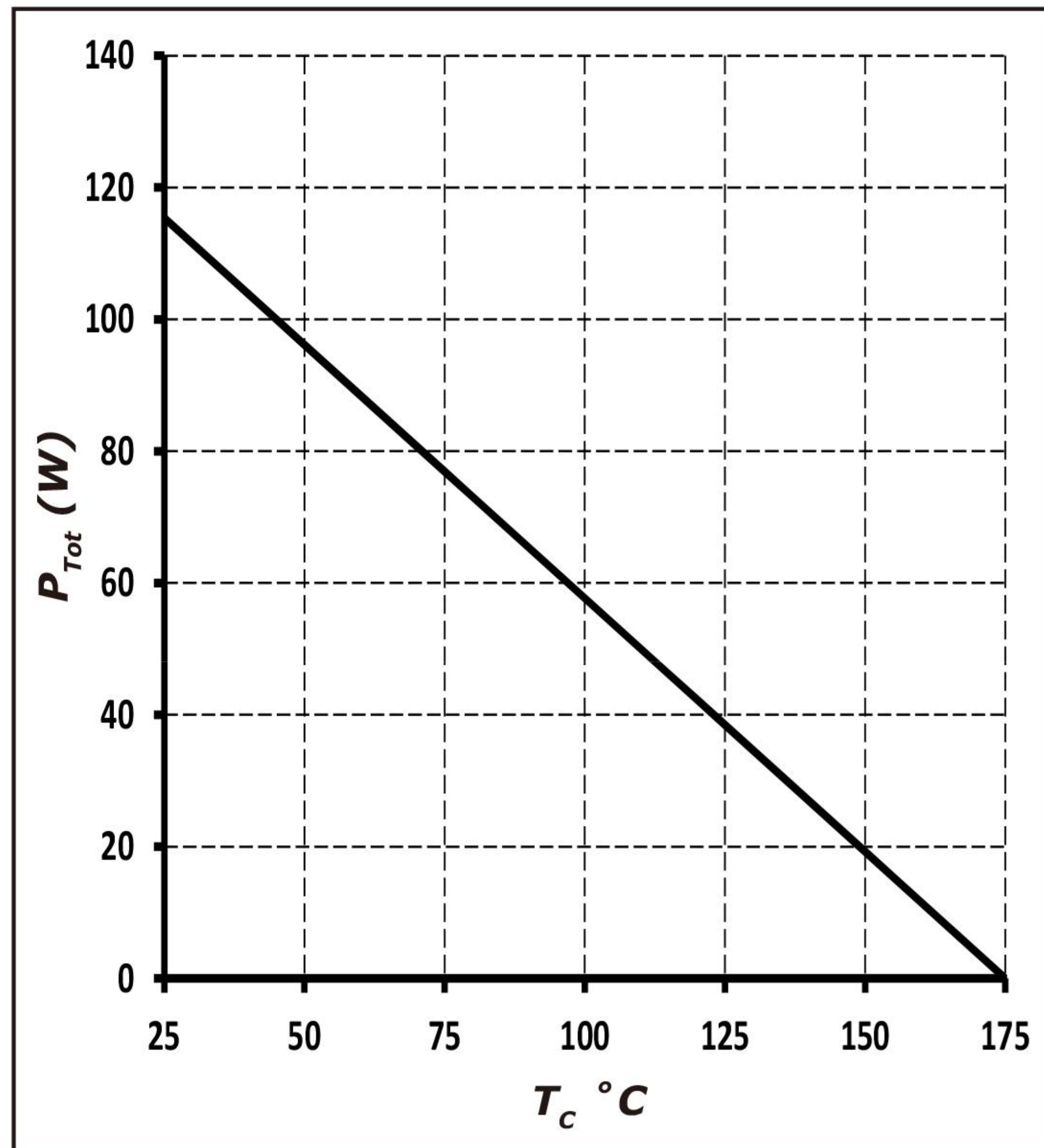
Figure 4. Power Derating
