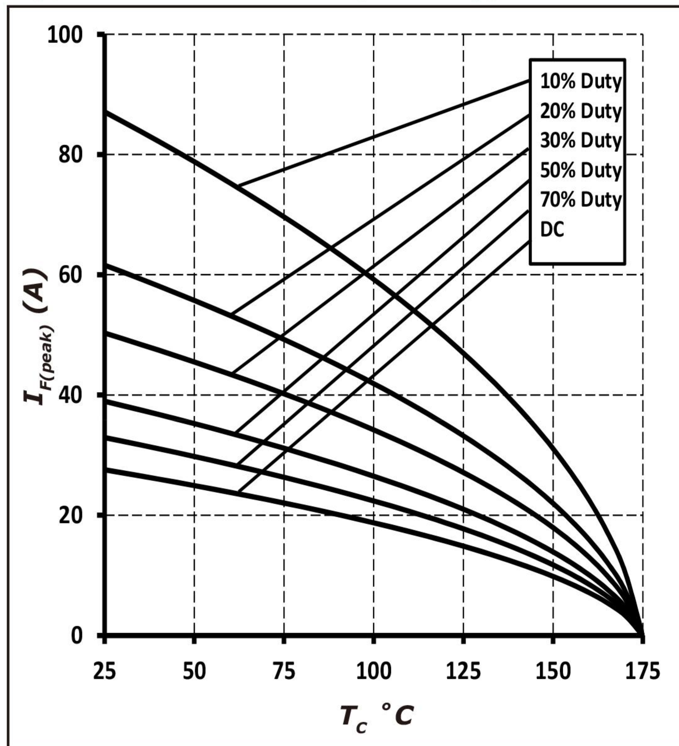
Figure 3. Current Derating
