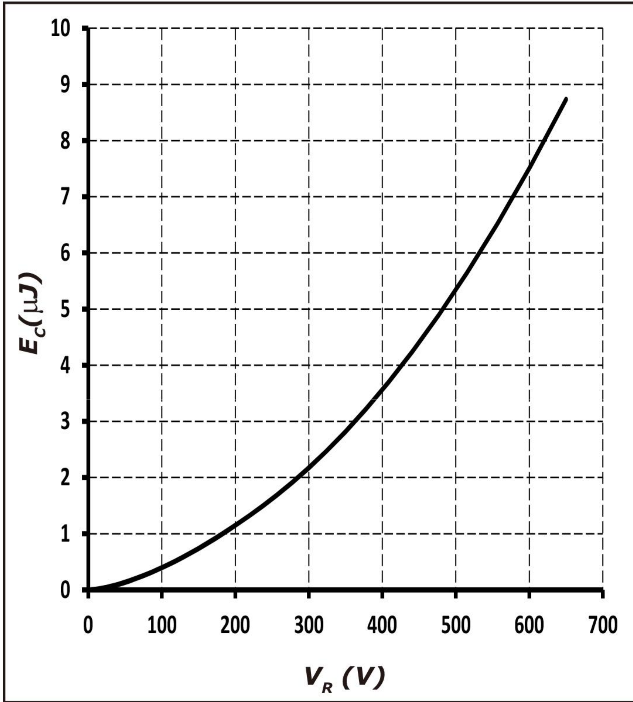
Figure 7. Capacitance Stored Energy
