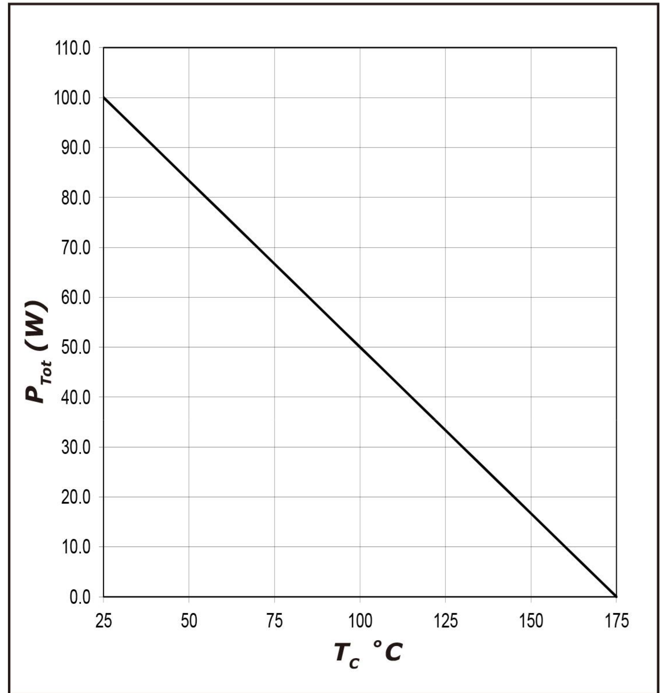
Figure 4. Power Derating
