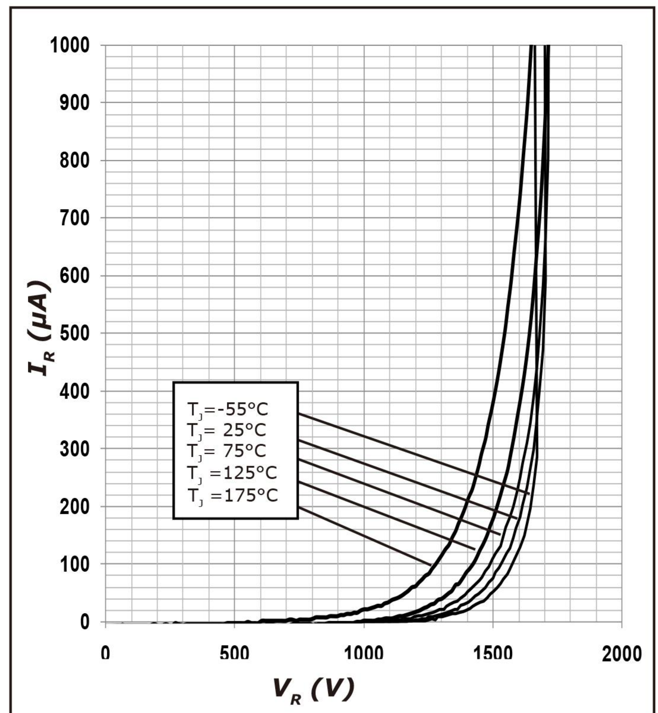
Figure 2. Reverse Characteristics
