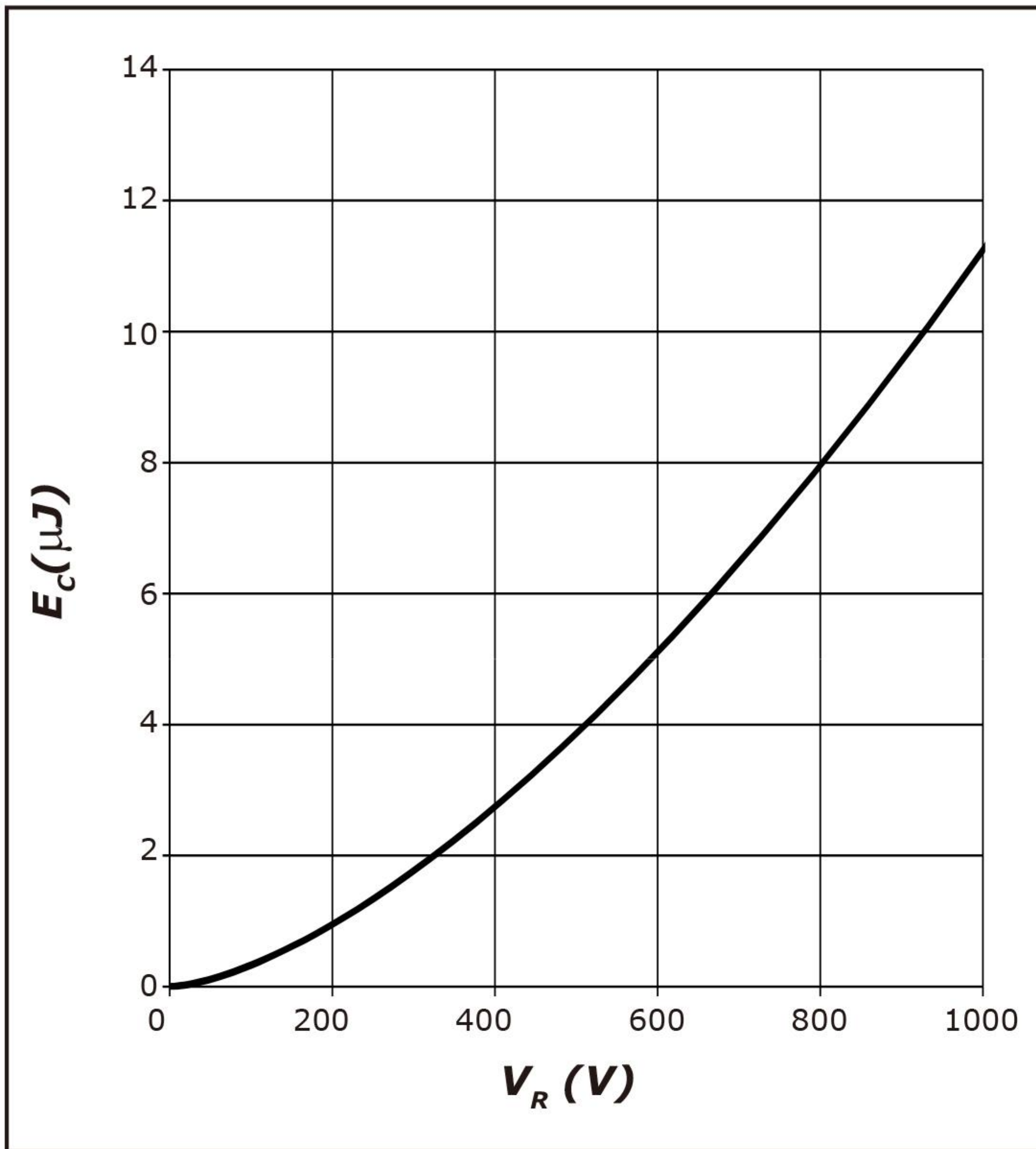
Figure 7. Typical Capacitance Stored Energy
