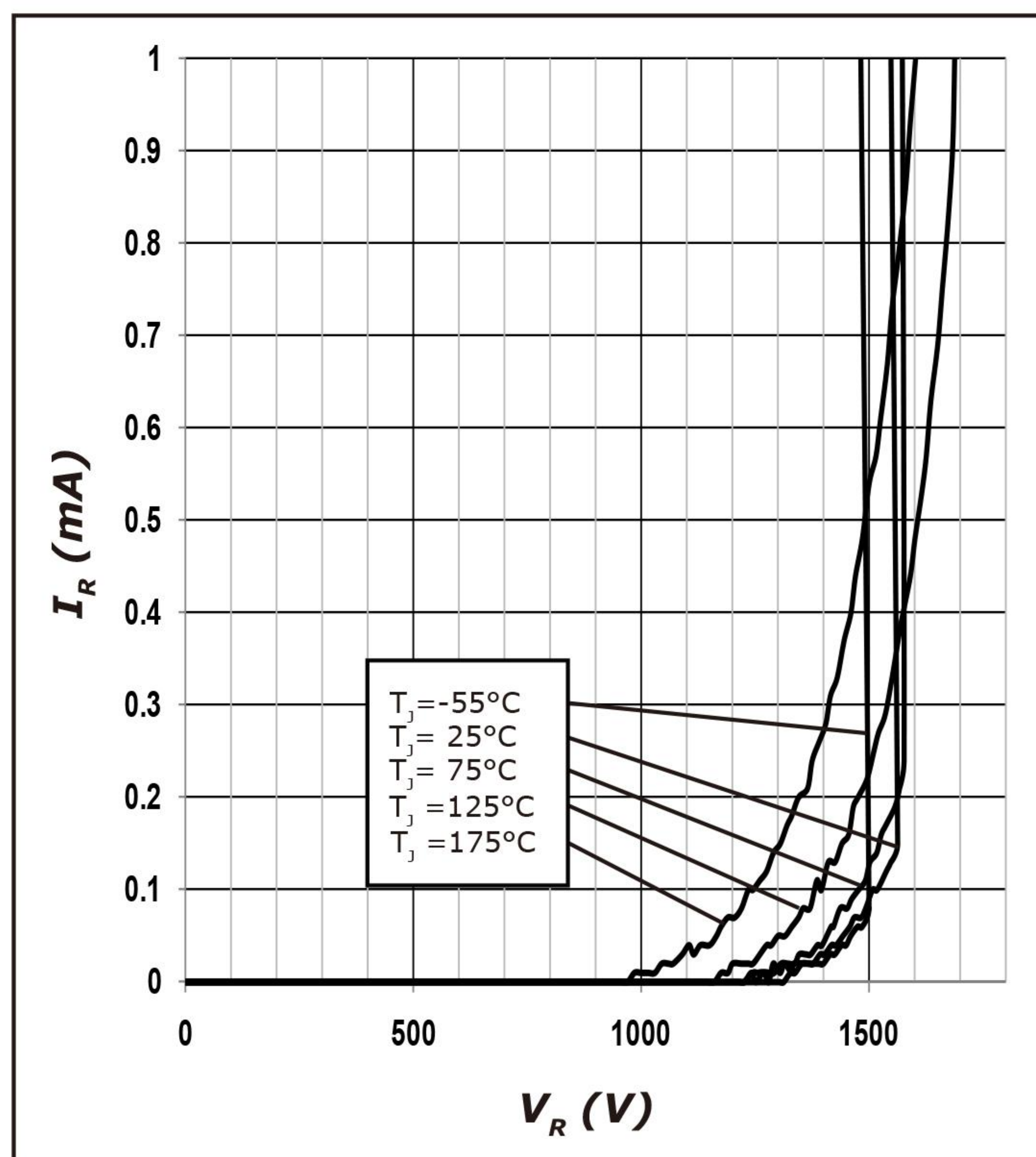
Figure 2. Reverse Characteristics
