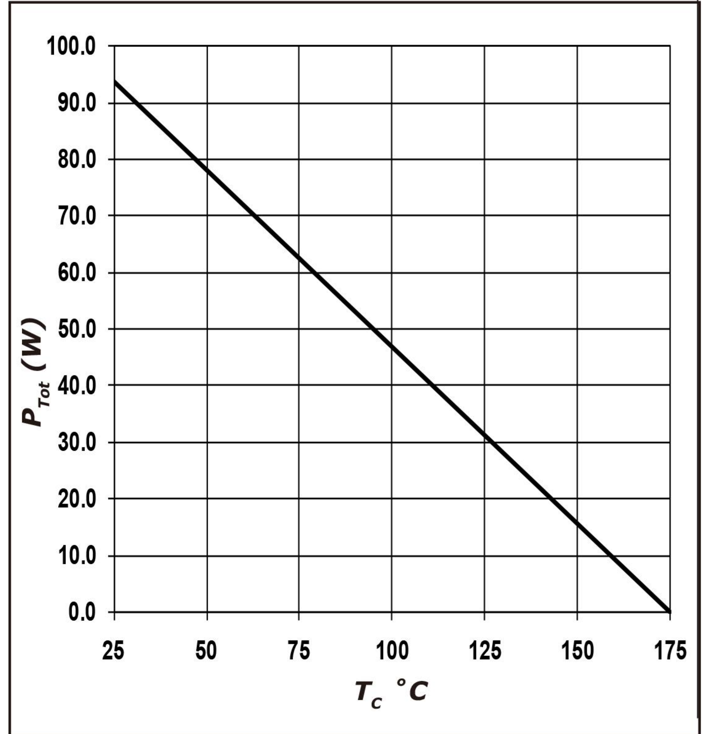
Figure 4. Power Derating
