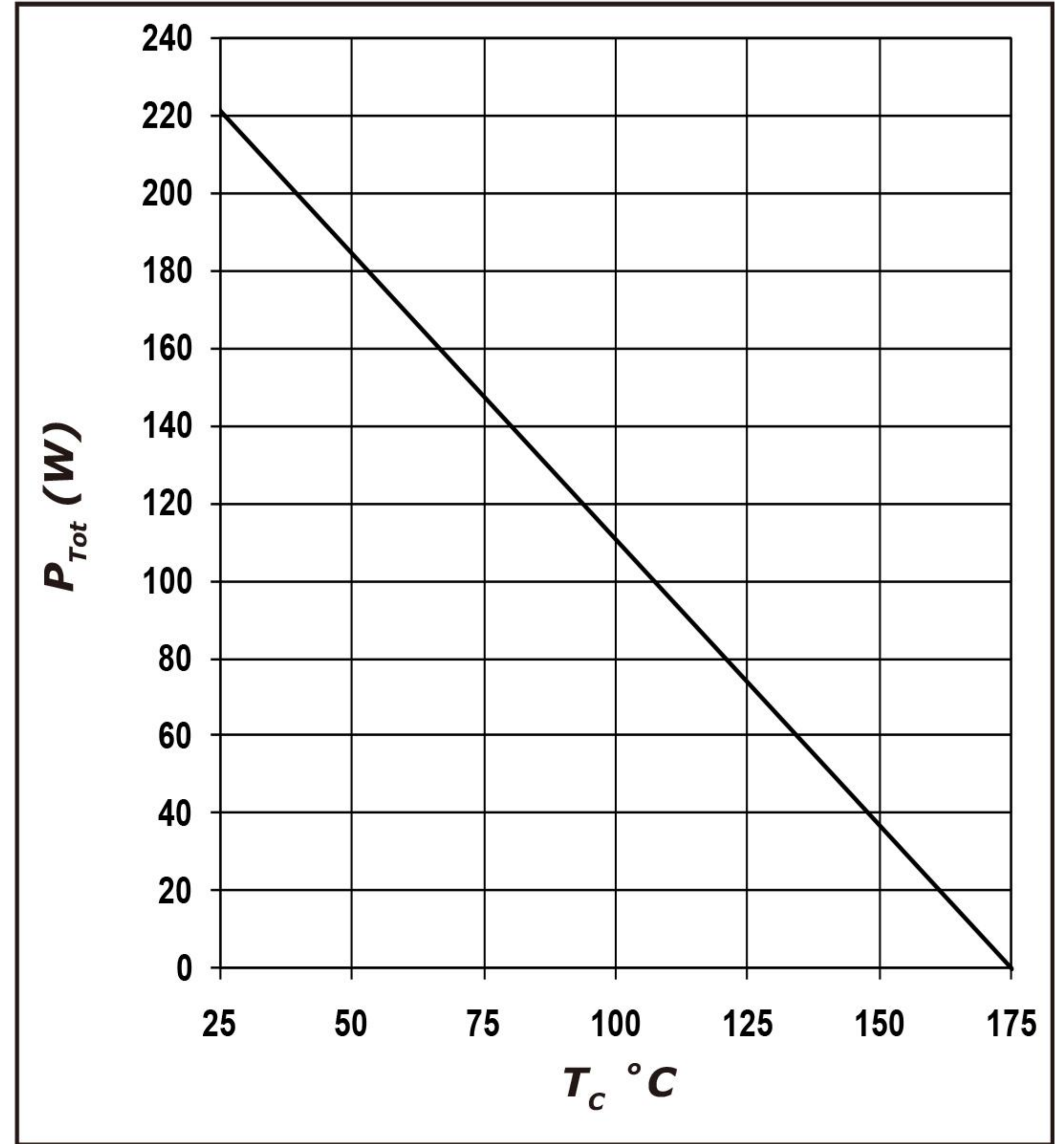
Figure 4. Power Derating
