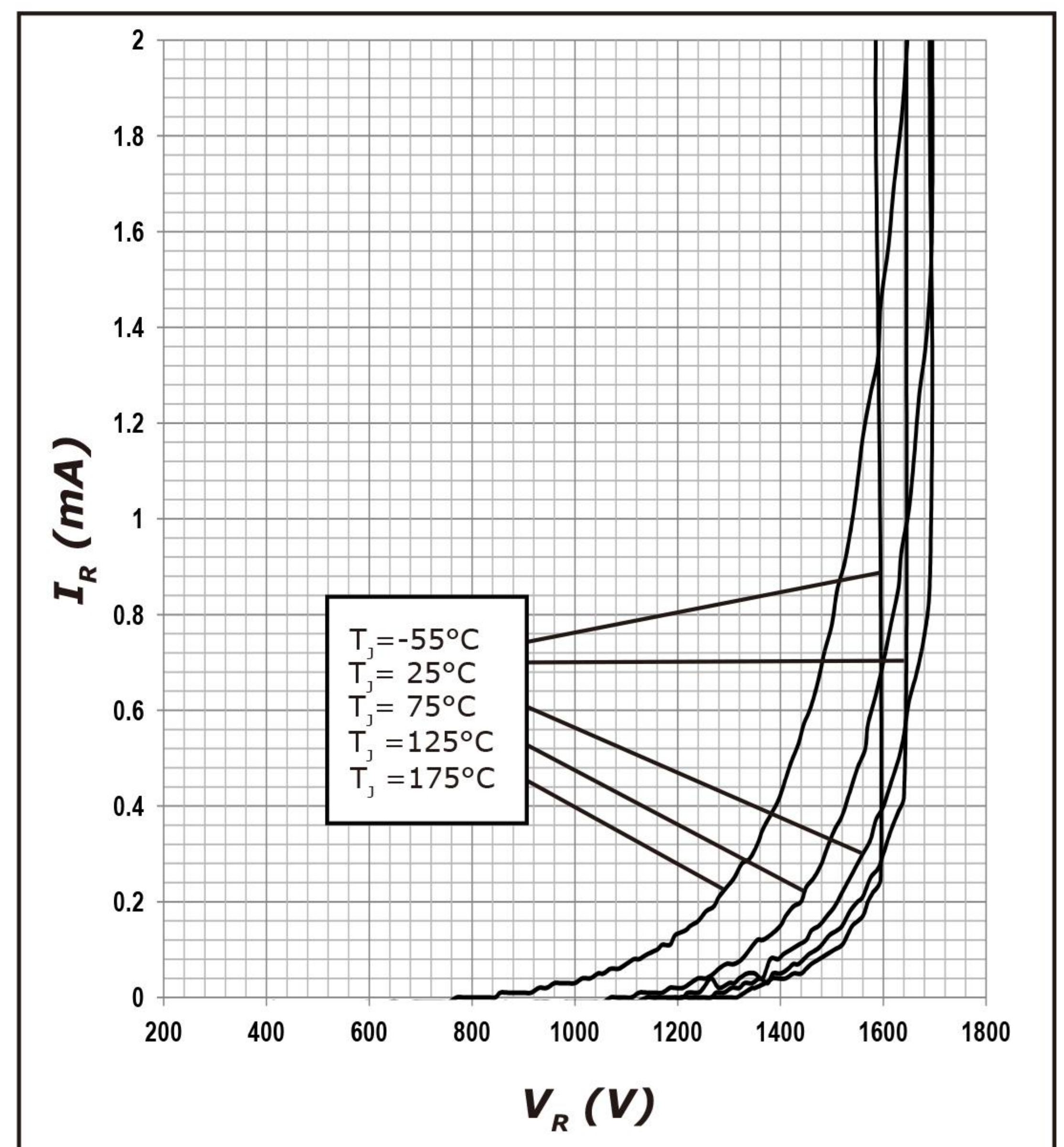
Figure 2. Reverse Characteristics
