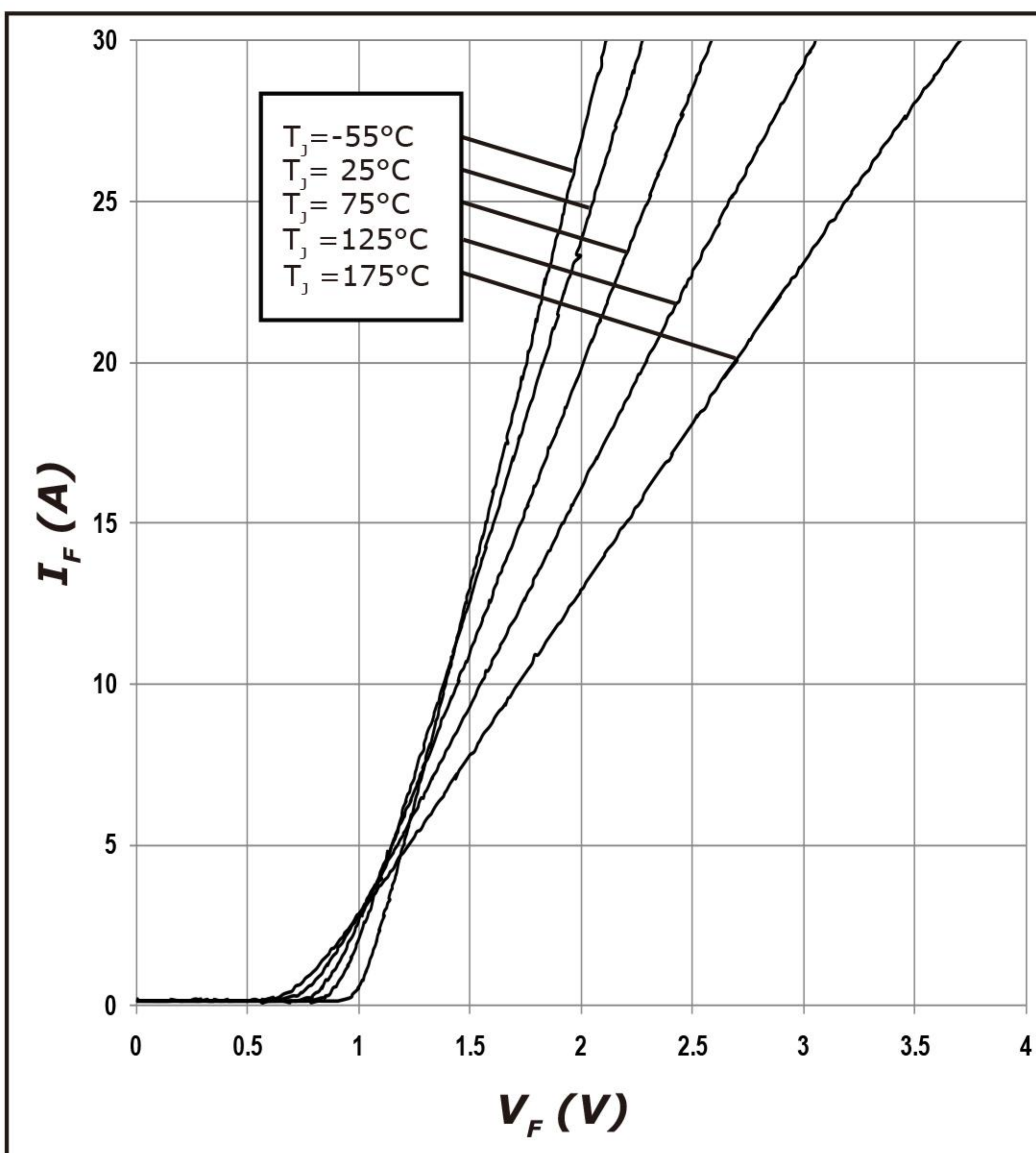
Figure 1. Forward Characteristics
