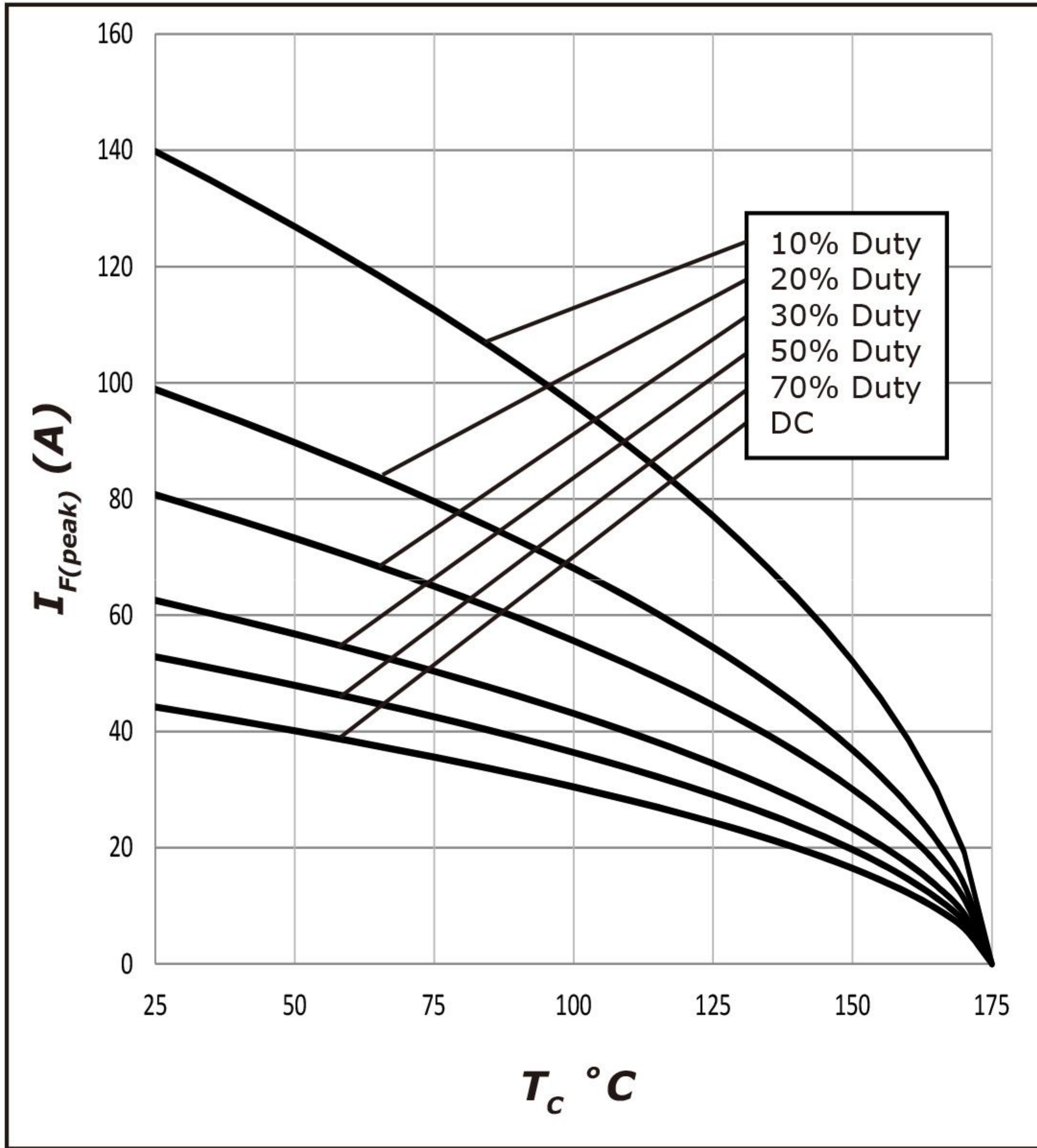
Figure 3. Current Derating
