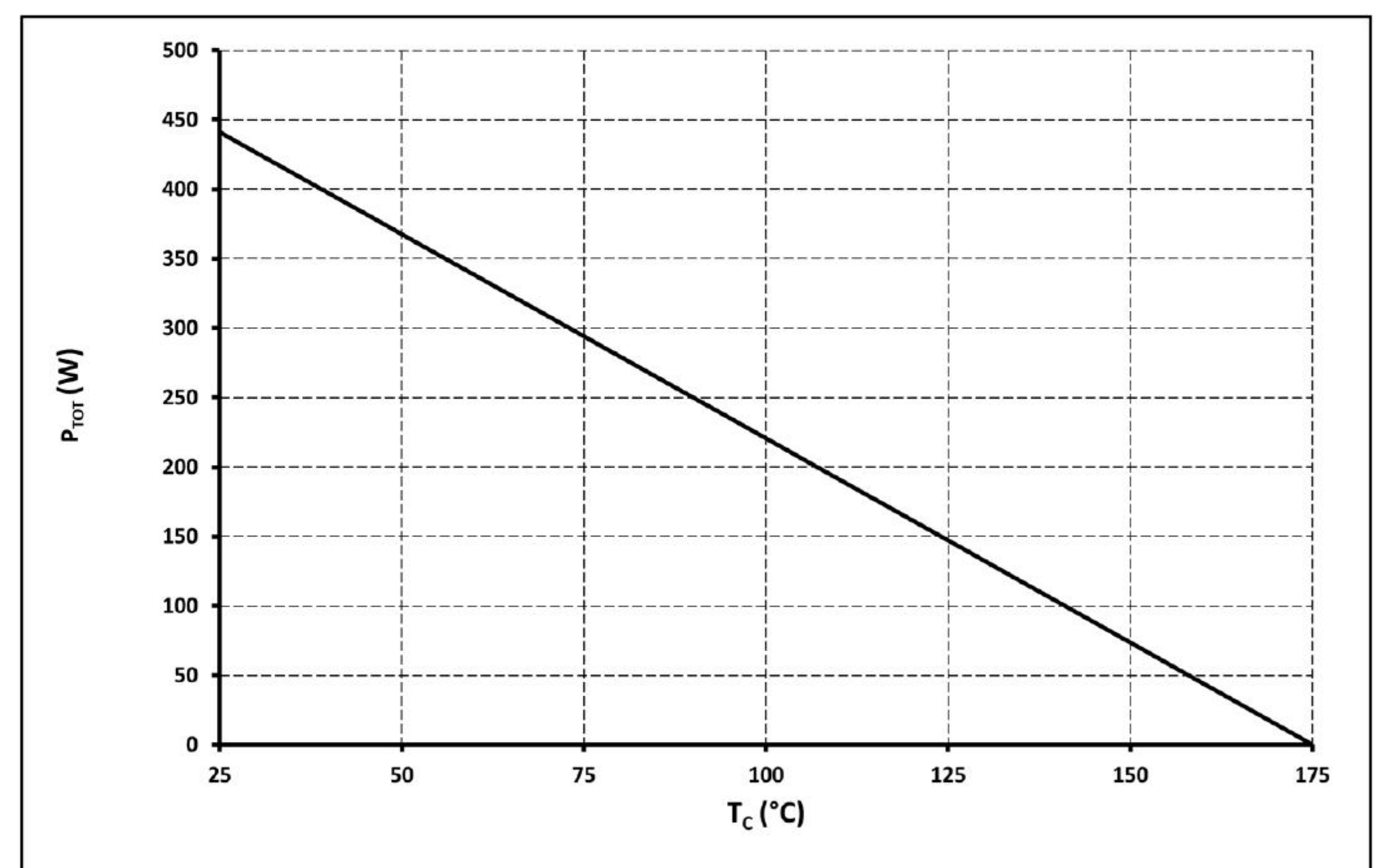
Figure 4. Power Derating
