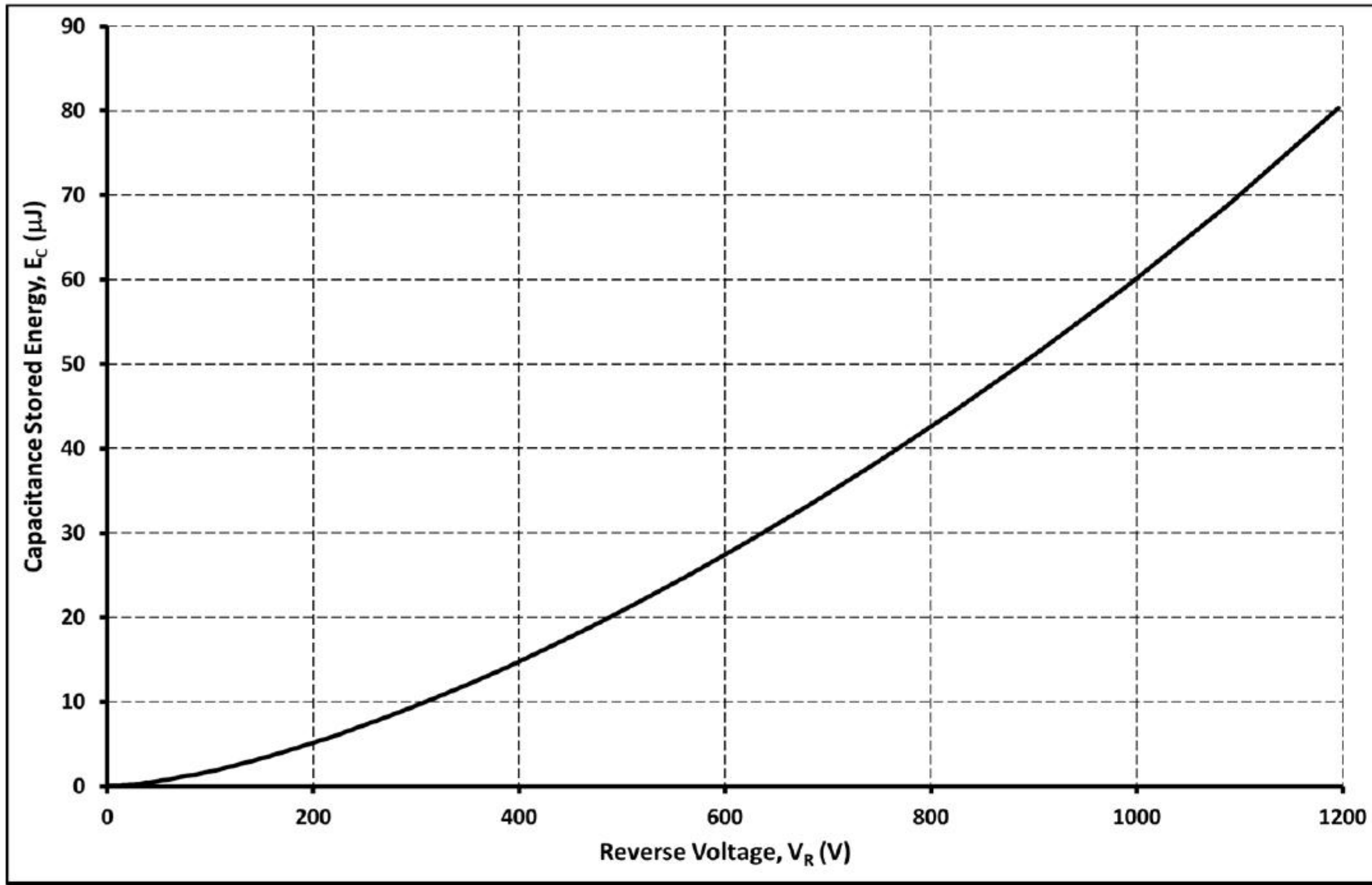
Figure 7. Capacitance Stored Energy
