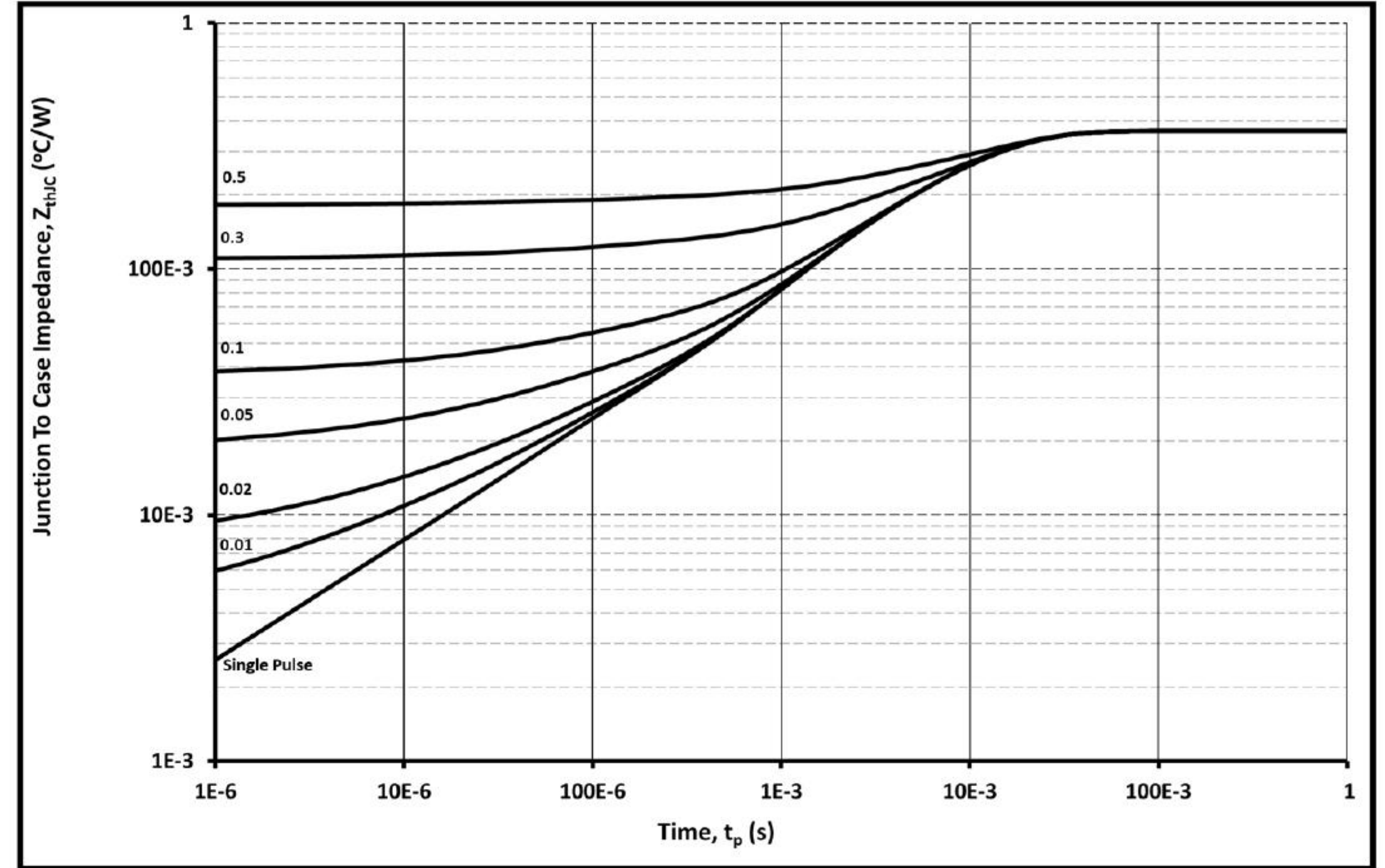
Figure 8. Transient Thermal Impedance
