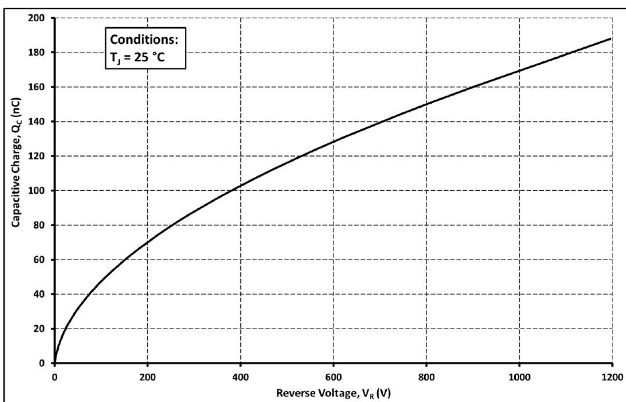
Figure 5. Total Capacitance Charge vs. Reverse Voltage
