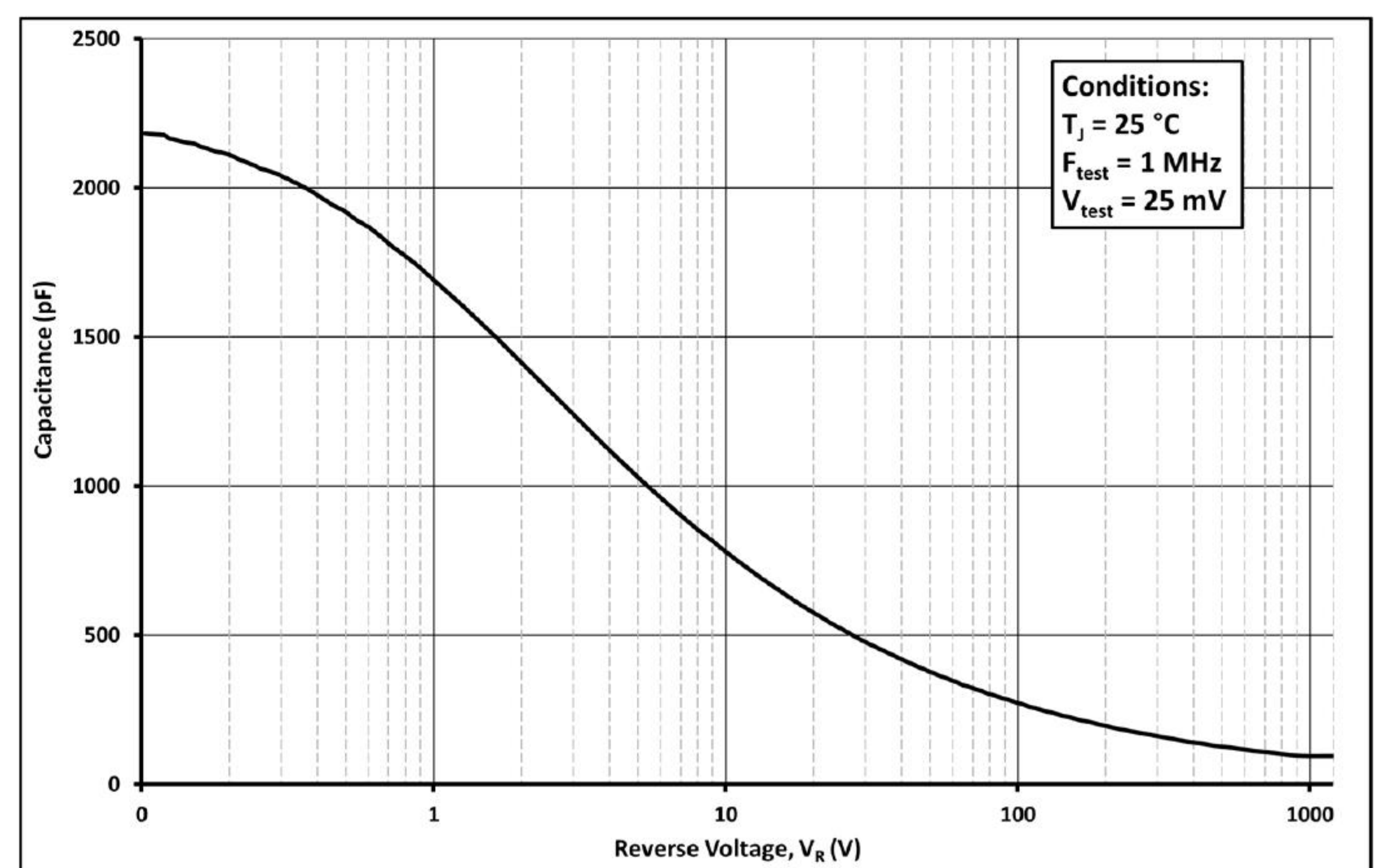
Figure 6. Capacitance vs. Reverse Voltage
