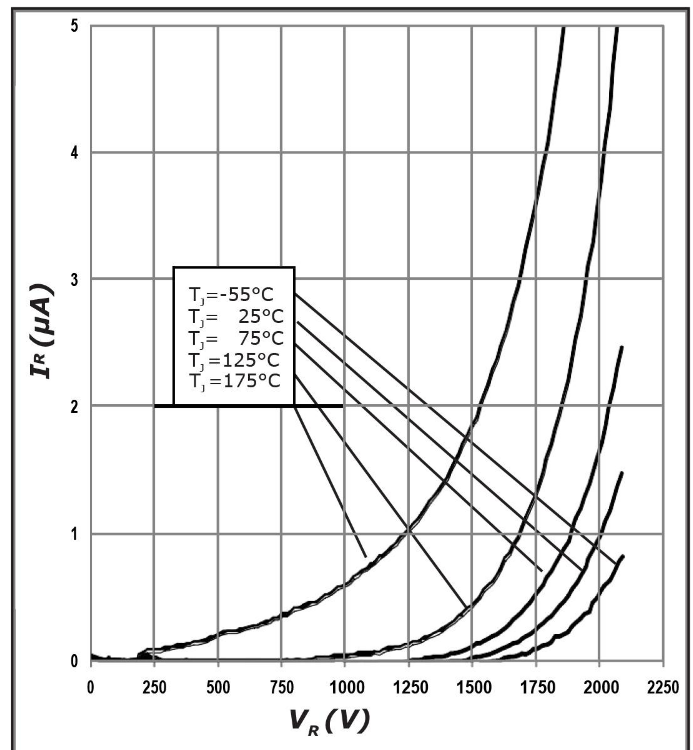
Figure 2. Reverse Characteristics
