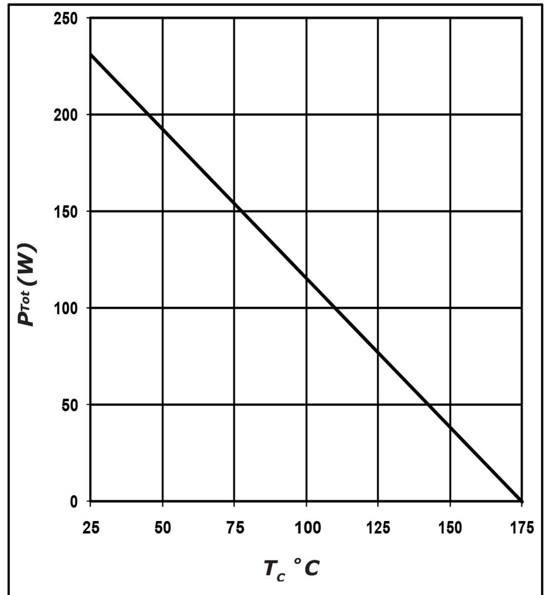
Figure 4. Power Derating
