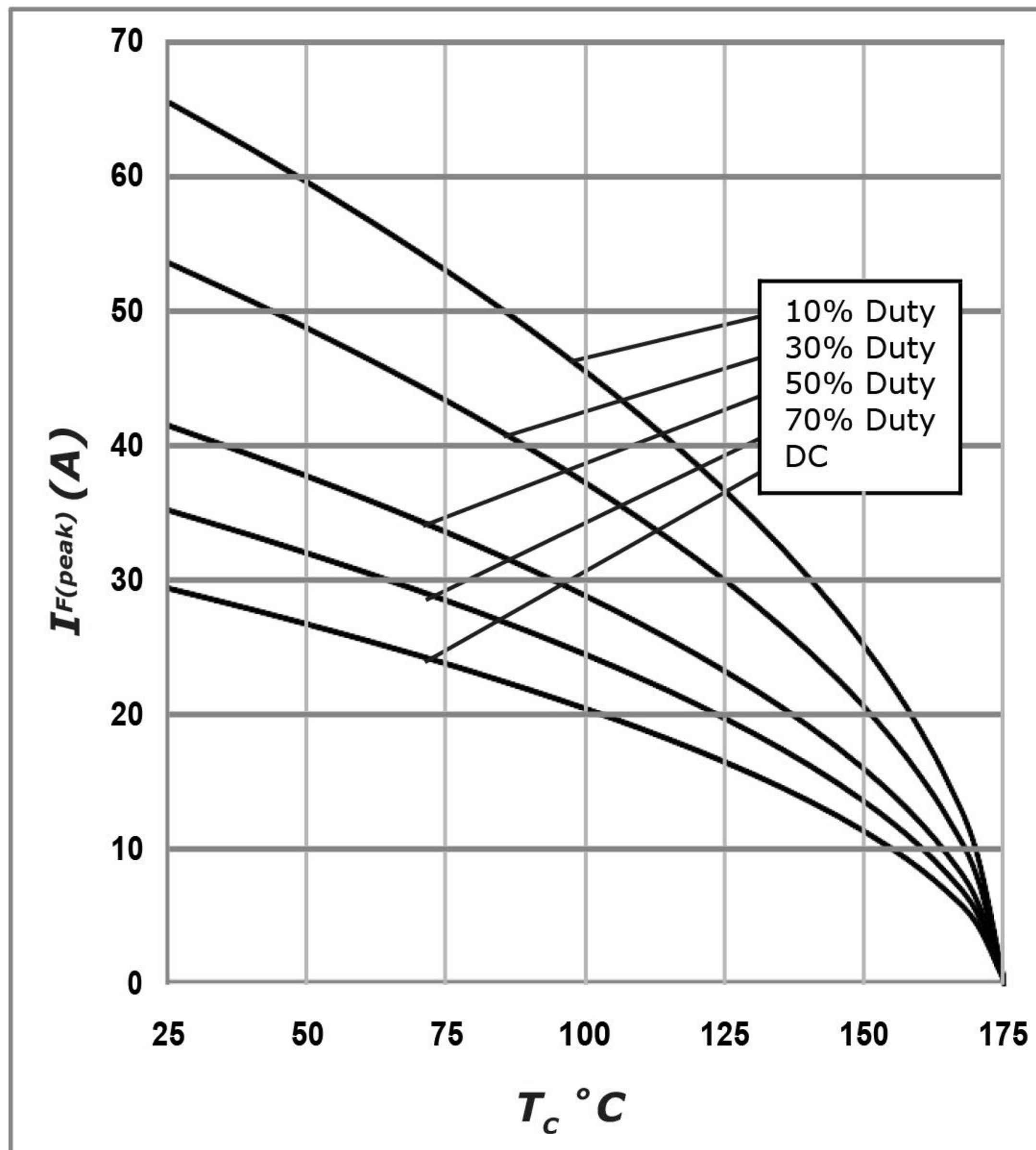
Figure 3. Current Derating
