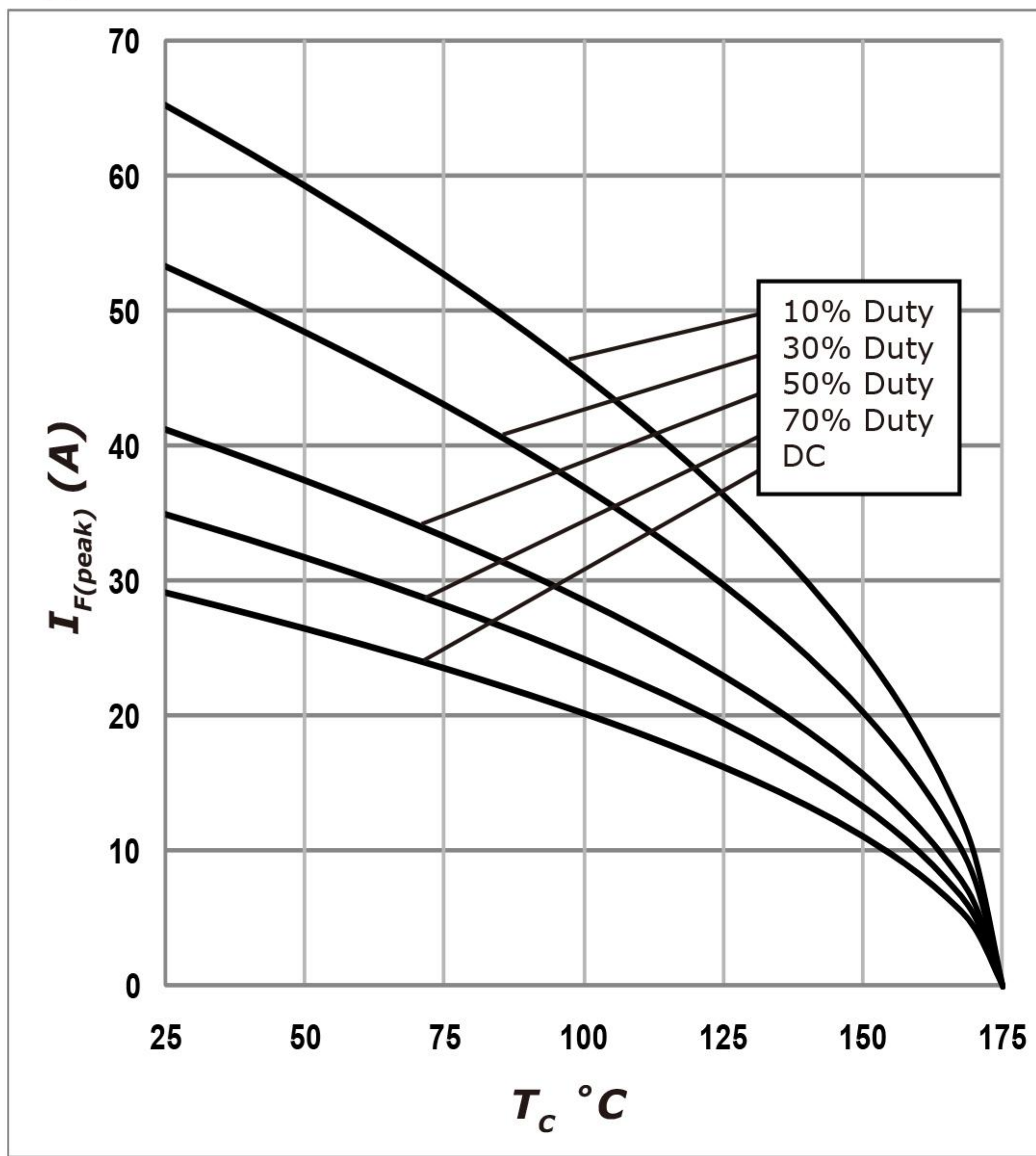
Figure 3. Current Derating
