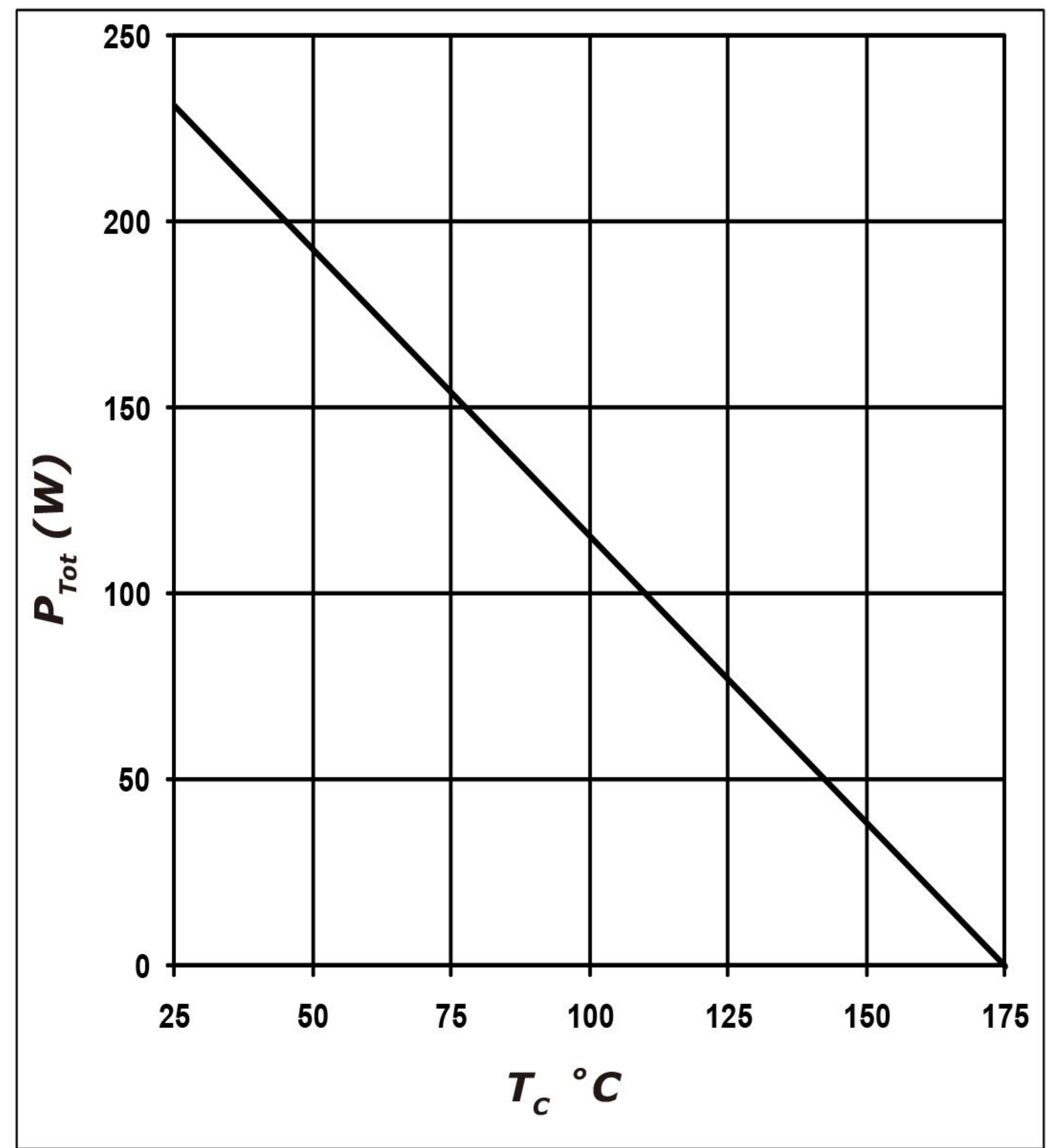
Figure 4. Power Derating
