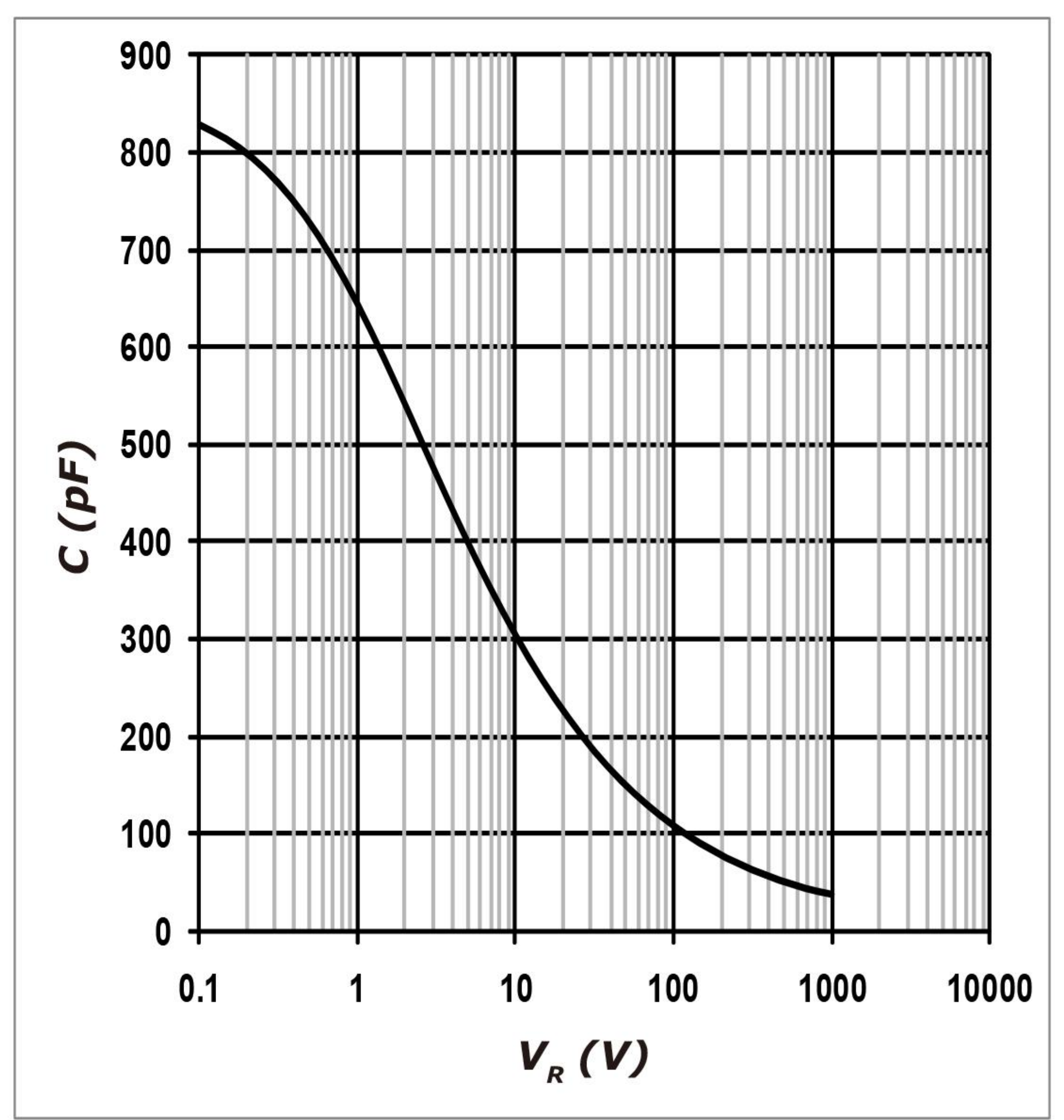
Figure 6. Capacitance vs. Reverse Voltage
