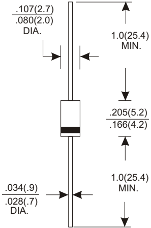
DO-41
